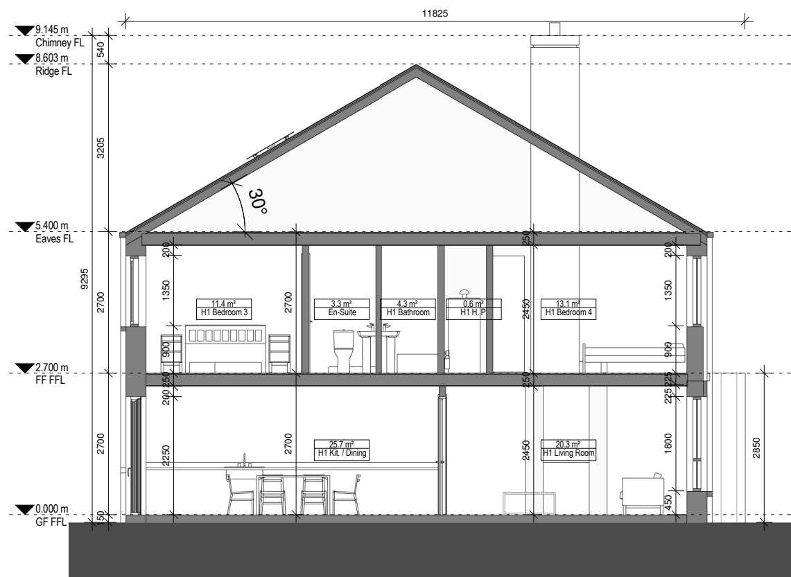
1 Section 1 1 : 100 @ A3
